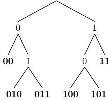
Figure 3.1: A prefix code represented as the leaves of a binary tree. This particular prefix code is given by \{00, 010, 011, 100, 101 \text{ and } 11.\}
