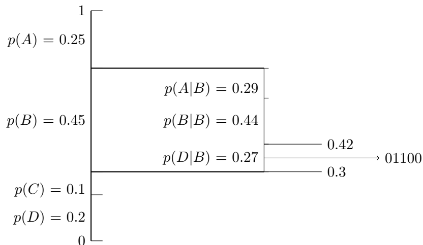
Figure 3.2: An arithmetic encoding of the sequence (B, D) gives string 01100. That p(C|B) = 0 is shown implicitly in second step.
